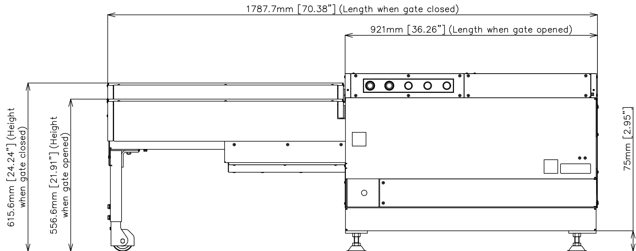
MODEL SOG2-F60-W060-H060-RG-CP
